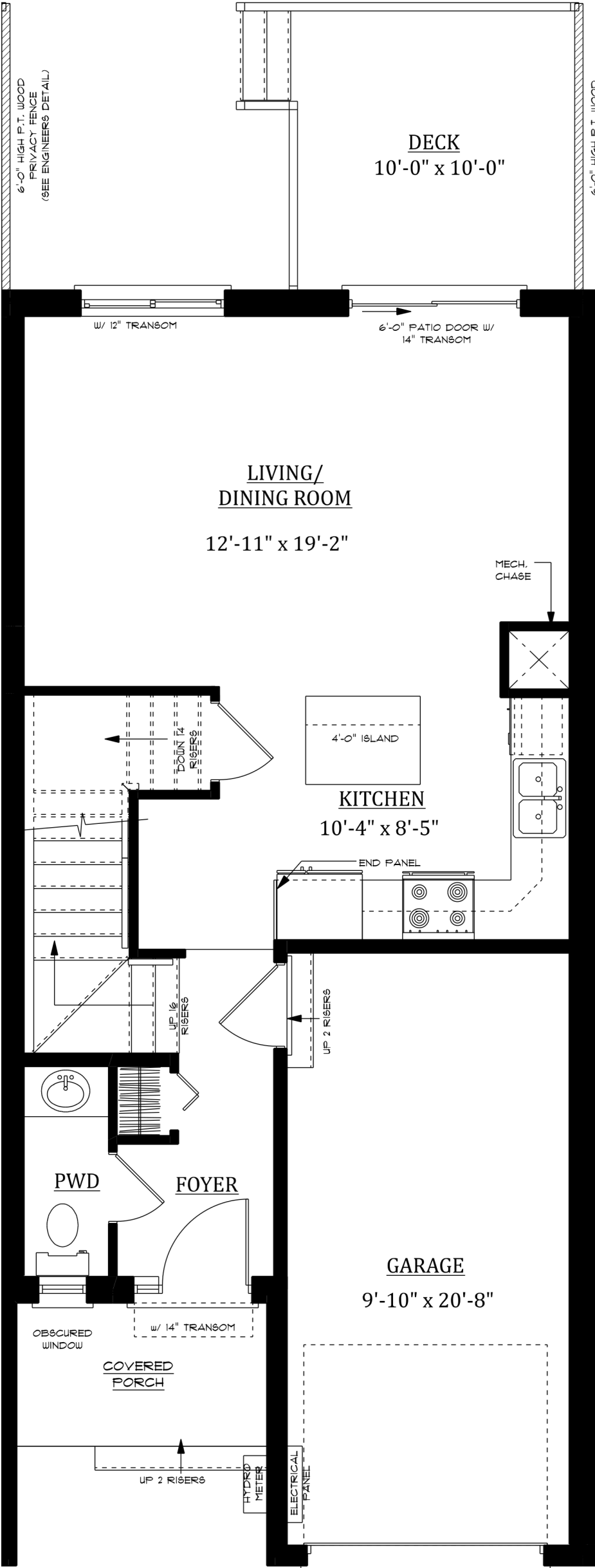
First Floor
