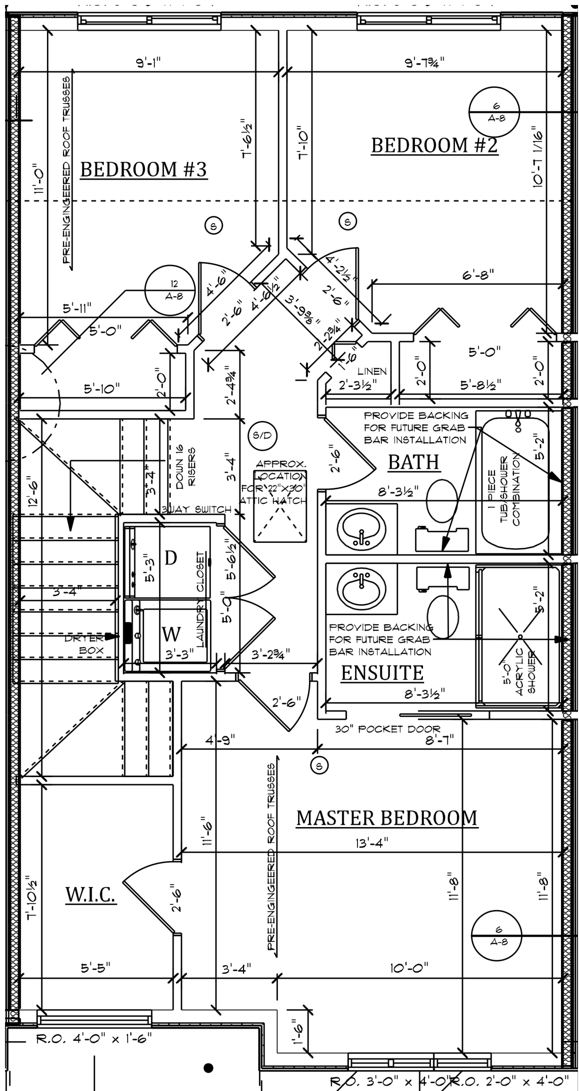
Second Floor
