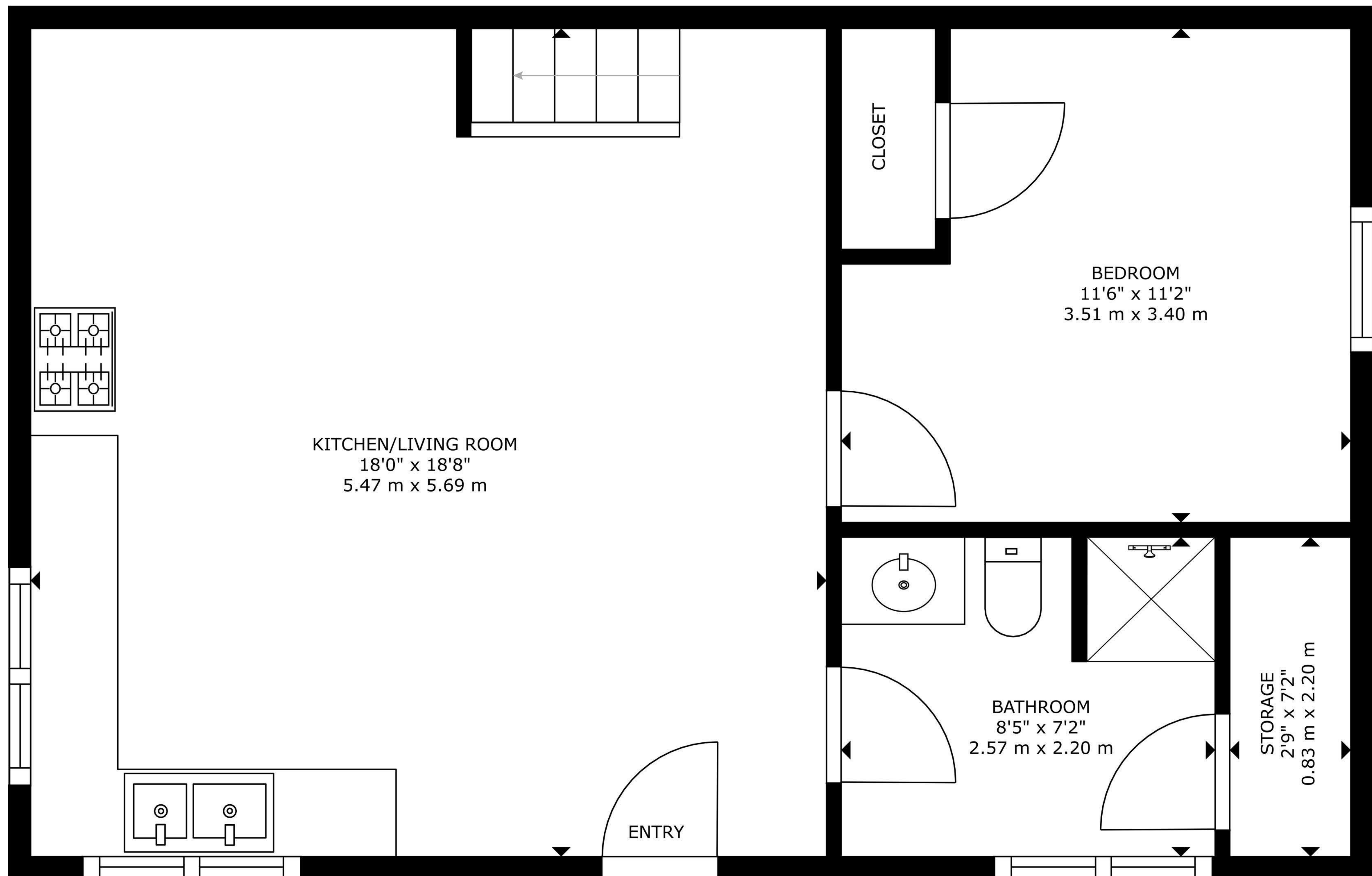
FLOOR PLAN
