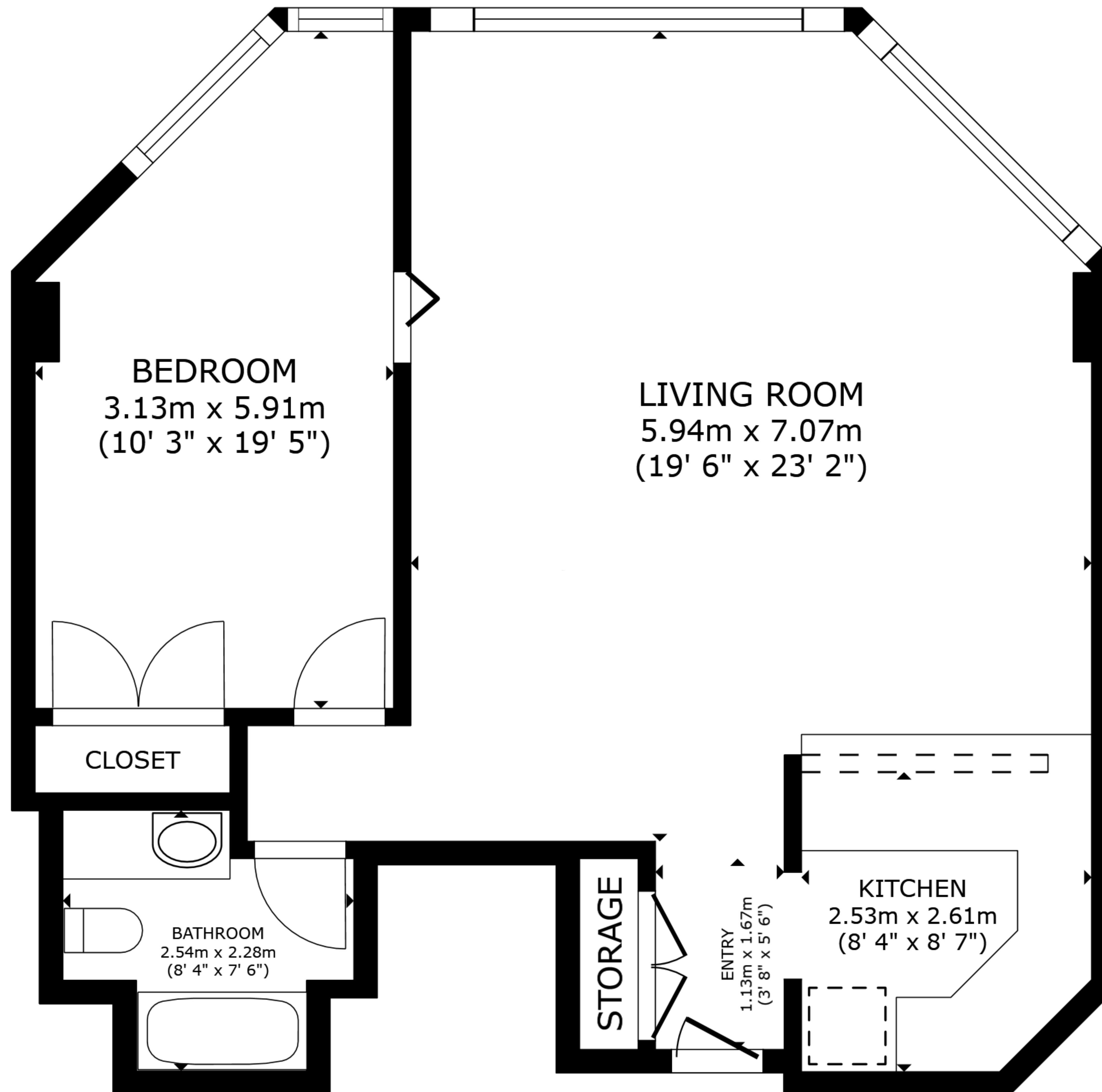
FLOOR PLAN
