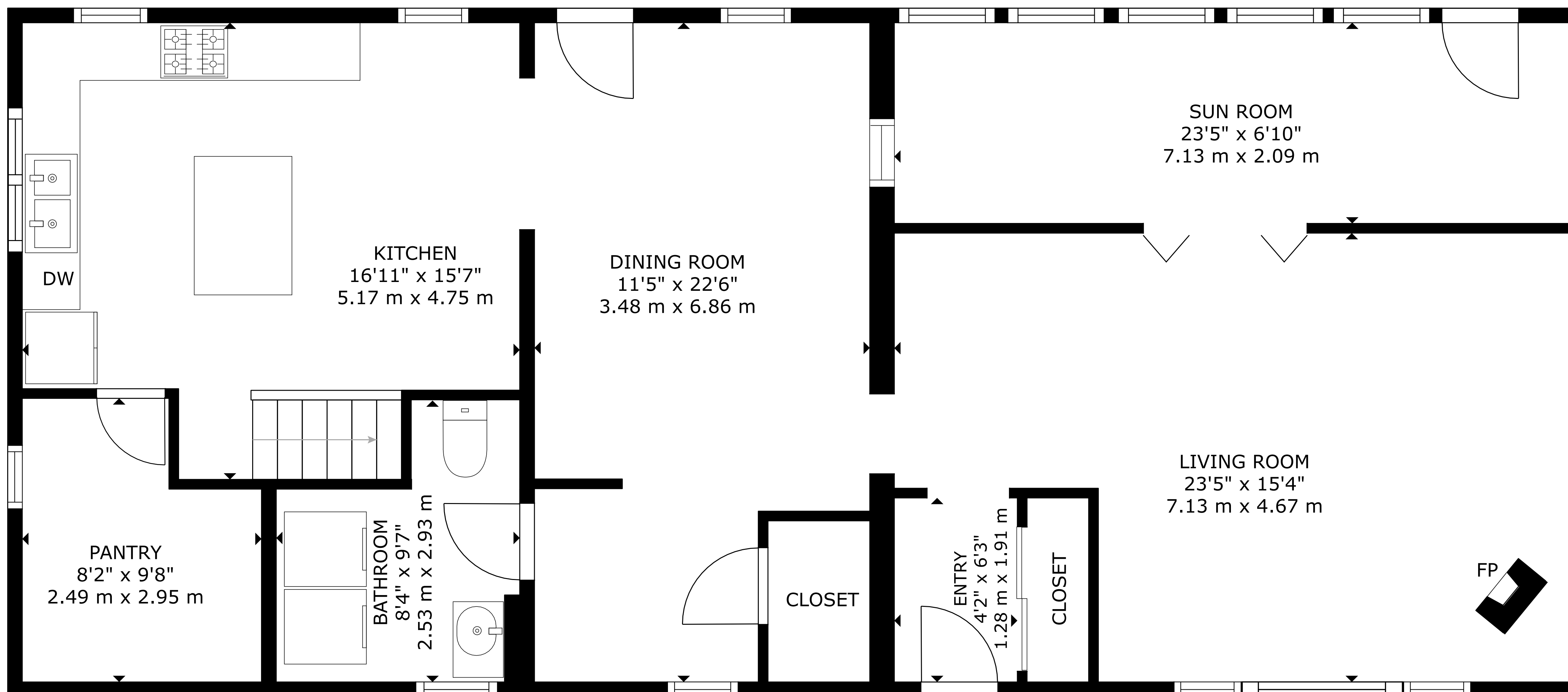
FLOOR 1
