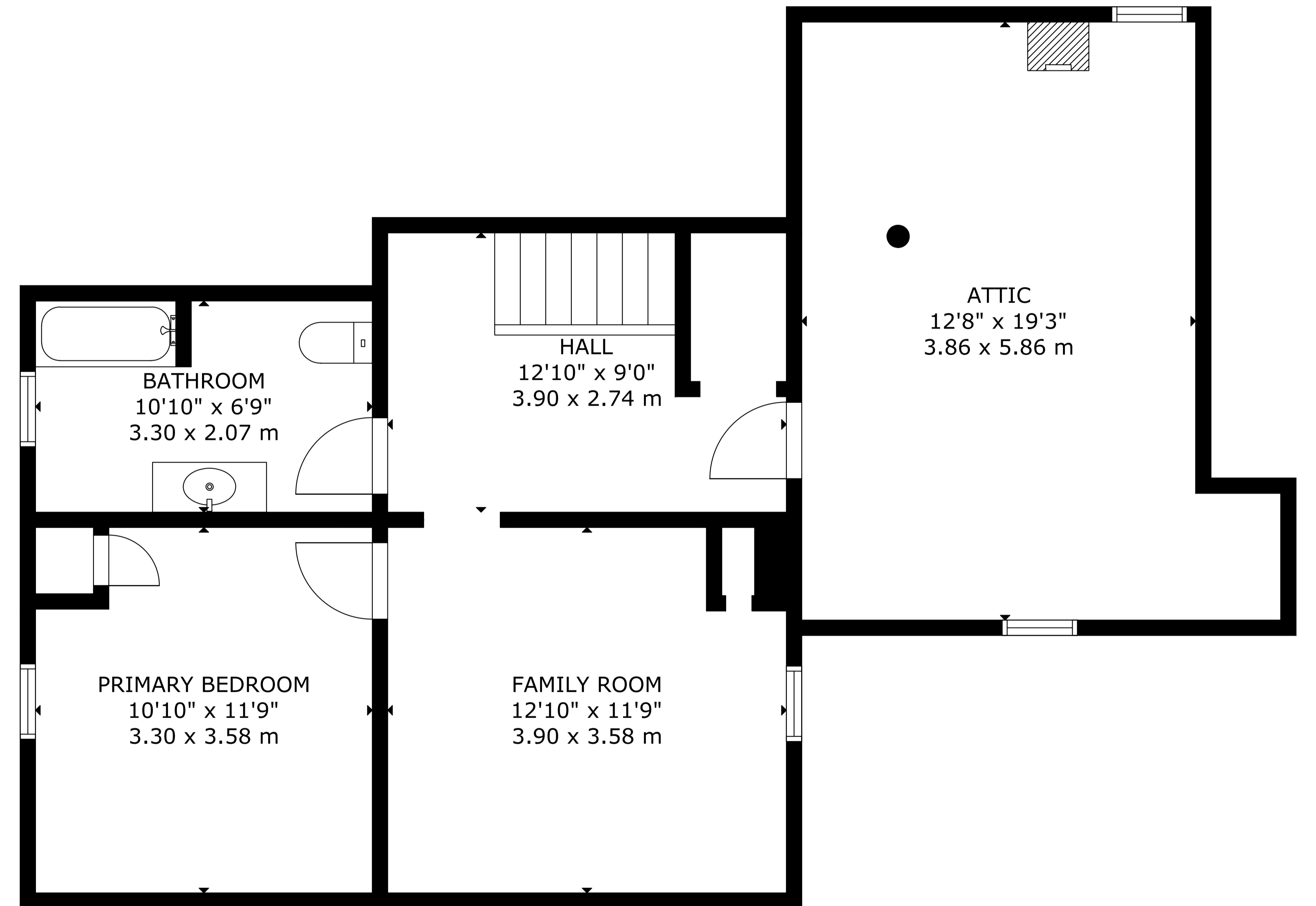
SECOND FLOOR
