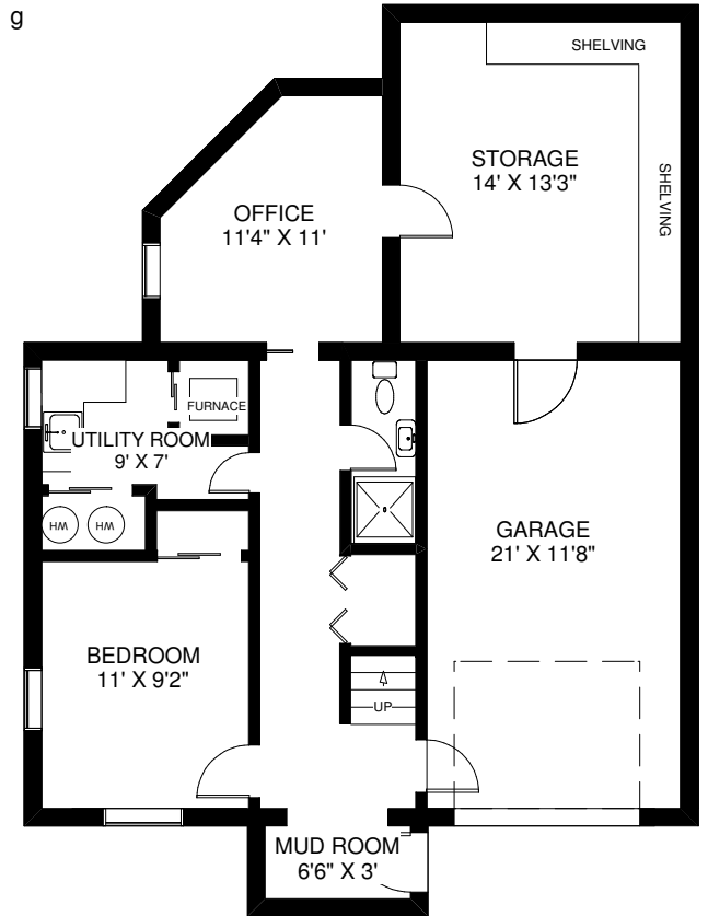
LOWER FLOOR APPROXIMATELY 900 SQ FT
