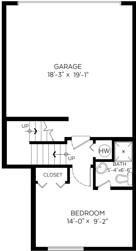
Lower Floor Plan Floor Area: 297 sq.ft.
