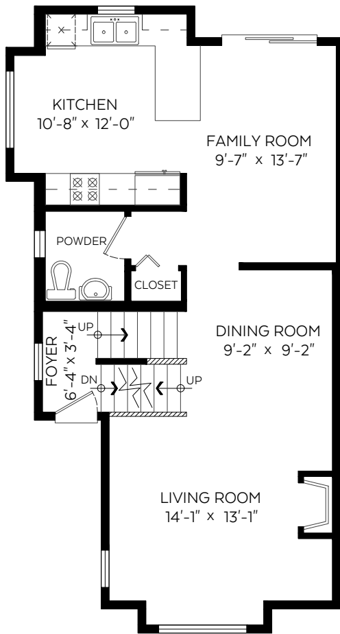
Main Floor Plan Floor Area: 698 sq.ft.
