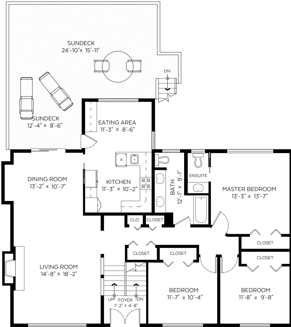
Main Floor Plan Floor Area: 1,522 sq.ft
