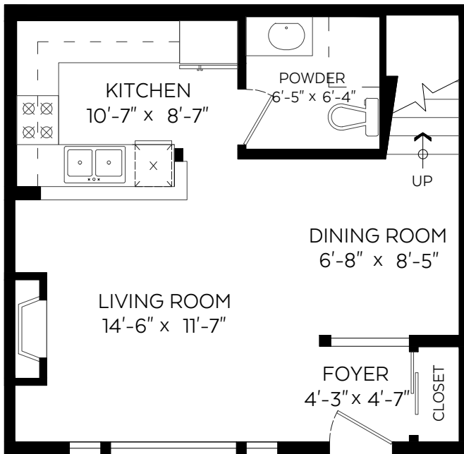
Main Floor Plan Floor Area: 476 sq.ft
