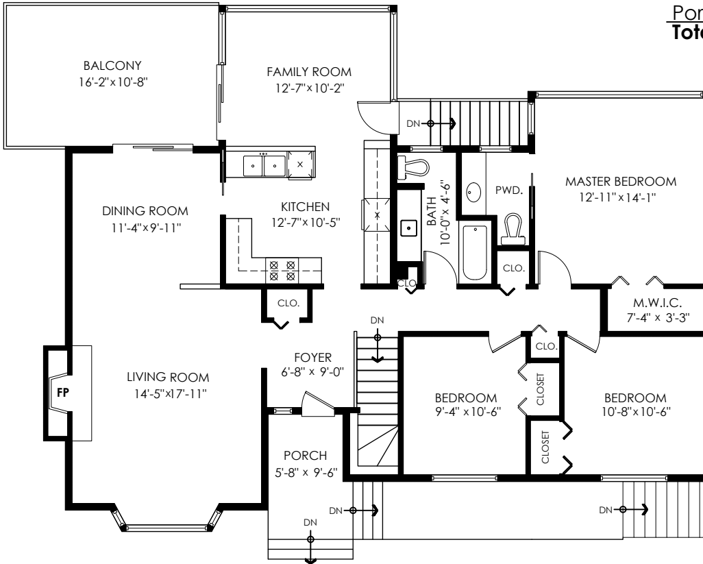
Main Floor Plan Floor Area: 1471 sq.ft. Ceiling Height: 8'-1"
