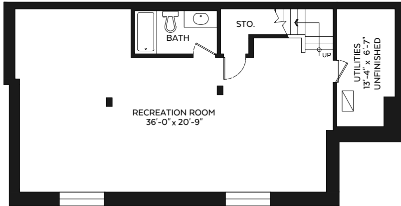
Lower Floor Plan Fin. Floor Area: 863 sq.ft. Unfin. Floor Area: 120 sq.ft. Ceiling Height: 8'-0"
