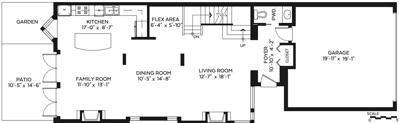
Main Floor Plan Floor Area: 973 sq.ft. Ceiling Height: 9'-0"
