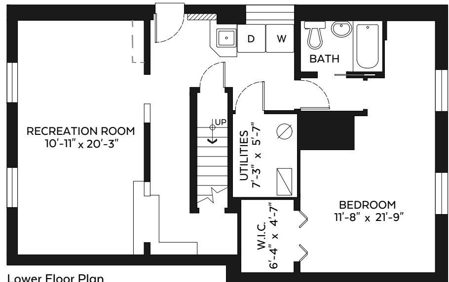
Lower Floor Plan Floor Area: 882 sq.ft.
