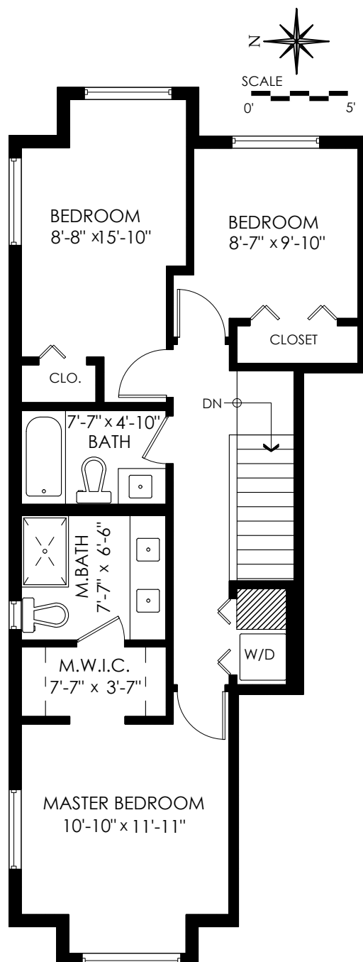
Upper Floor Plan
