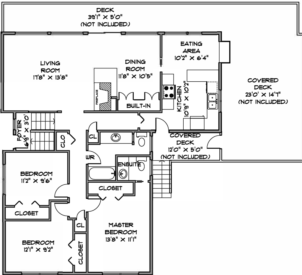
MAIN LEVEL 1393 SQ. FT.
