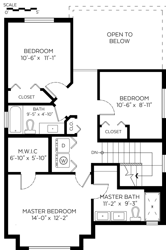
Upper Floor Plan Floor Area: 866 sq.ft.
