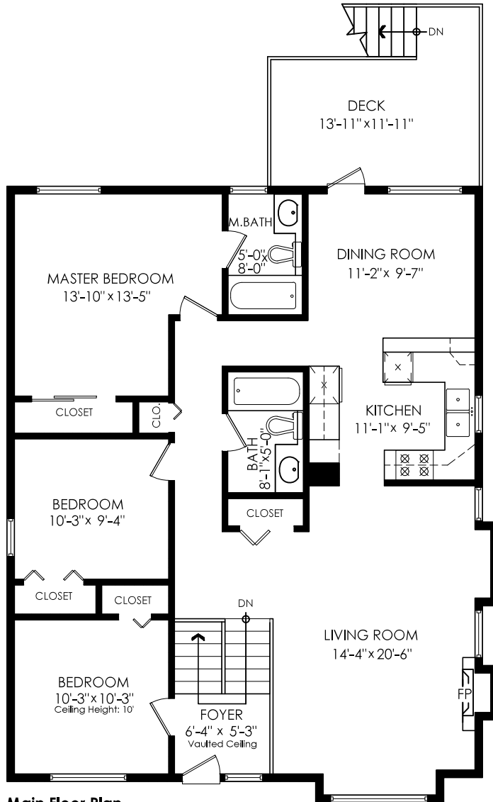
Main Floor Plan Floor Area: 1269 sq.ft. Ceiling Height: 8'-0"
