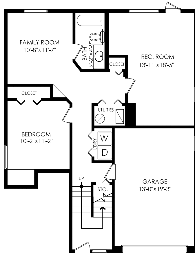
Lower Floor Plan Floor Area: 850 sq.ft. Ceiling Height: 7'-11"
