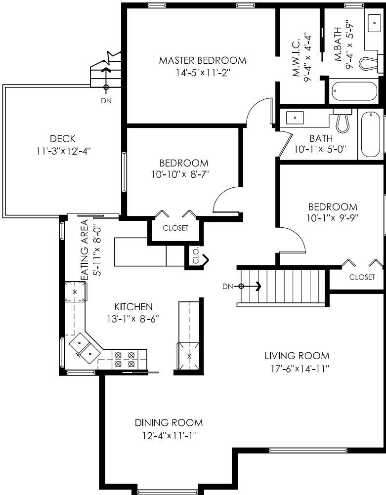
Main Floor Plan Floor Area: 1287 sq.ft. Ceiling Height: 8'
