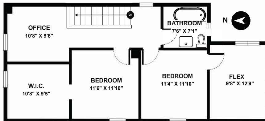
Upper Floor: 883 sqft Ceiling Height: 8'4"
