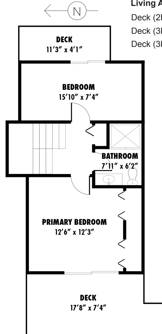
Upper Floor: 473 sq.ft. Ceiling Height: 7' 11" - 11'0"
