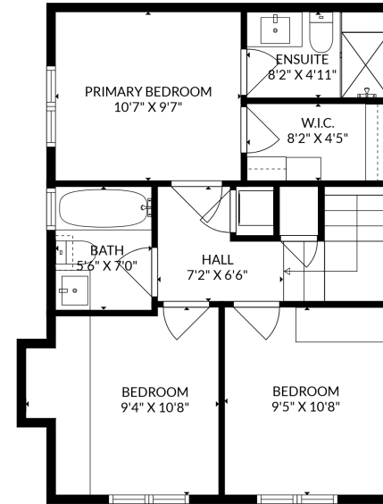
Upper Floor: 577 sq.ft.
