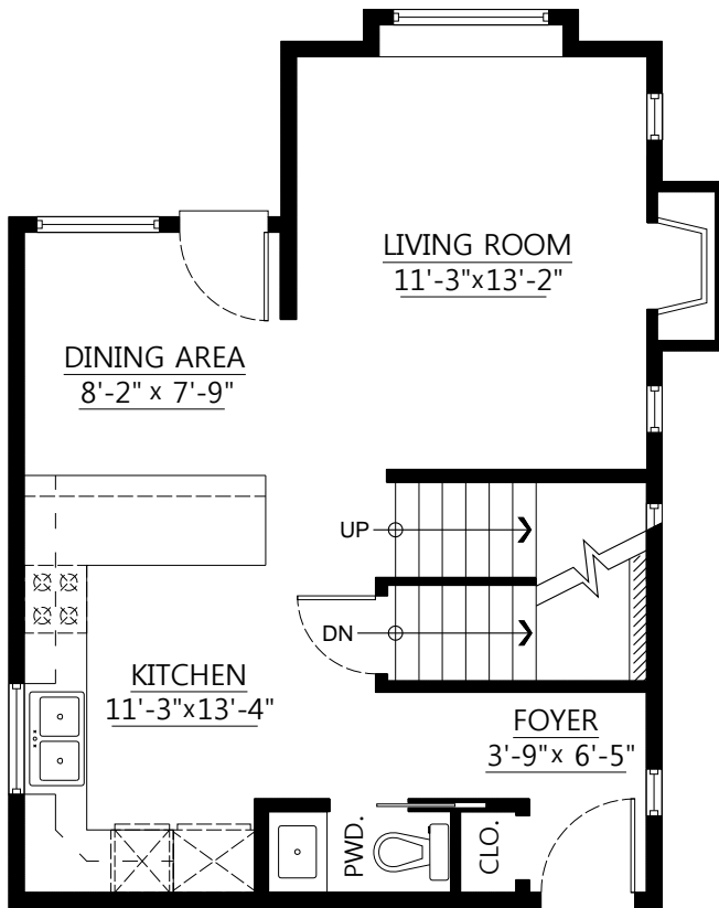
Main Floor Plan Floor Area: 531 sq.ft.
