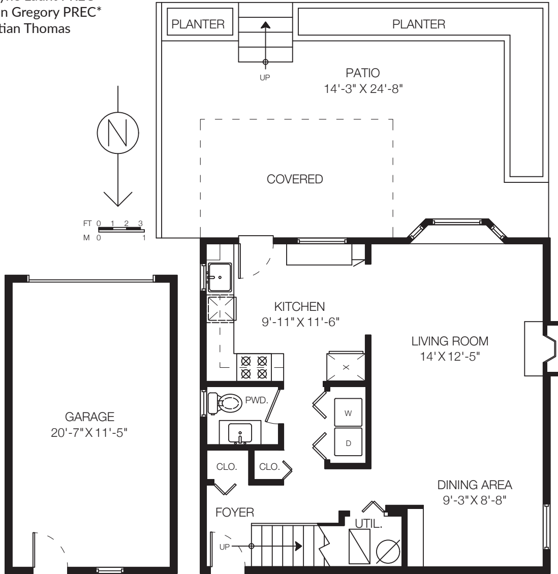
Main Floor: 610 Sq.Ft. Ceiling Height: 8'
