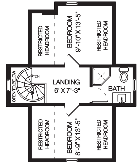
Top Floor: 239 Sq.Ft. Ceiling Height: 8'
