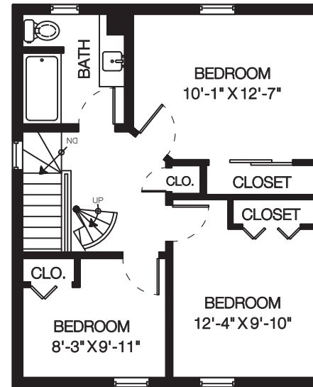
Upper Floor: 569 Sq.Ft. Ceiling Height: 9'
