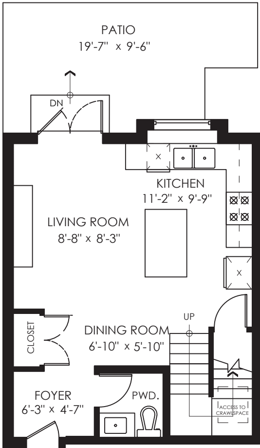
Main Floor: 478 Sq.Ft. Ceiling Height: 9'-0"
