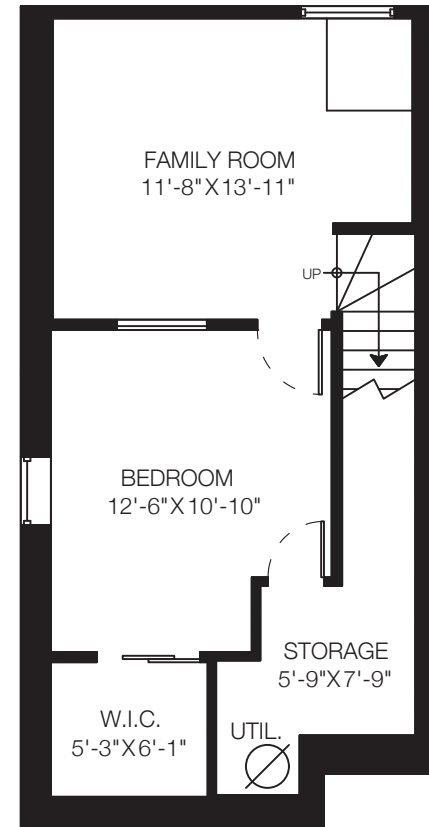
Lower Floor: 508 Sq.Ft. Ceiling Height: 8'
