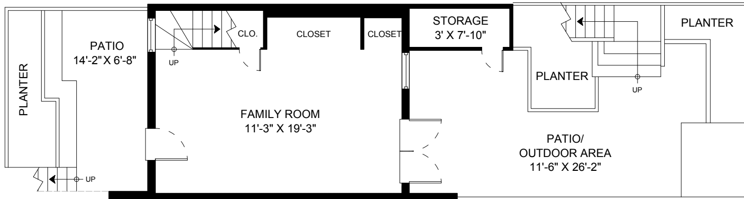
Lower Floor: 312 Sq.Ft. Ceiling Height: 7'-4"
