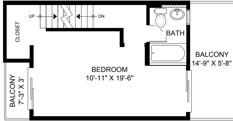
Upper Floor: 340 Sq.Ft. Ceiling Height: 7'-5"
