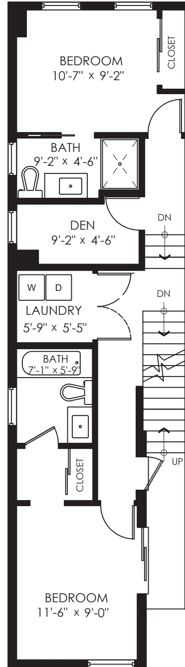
Top Floor: 631 Sq.Ft. Ceiling Height: 7'-11"
