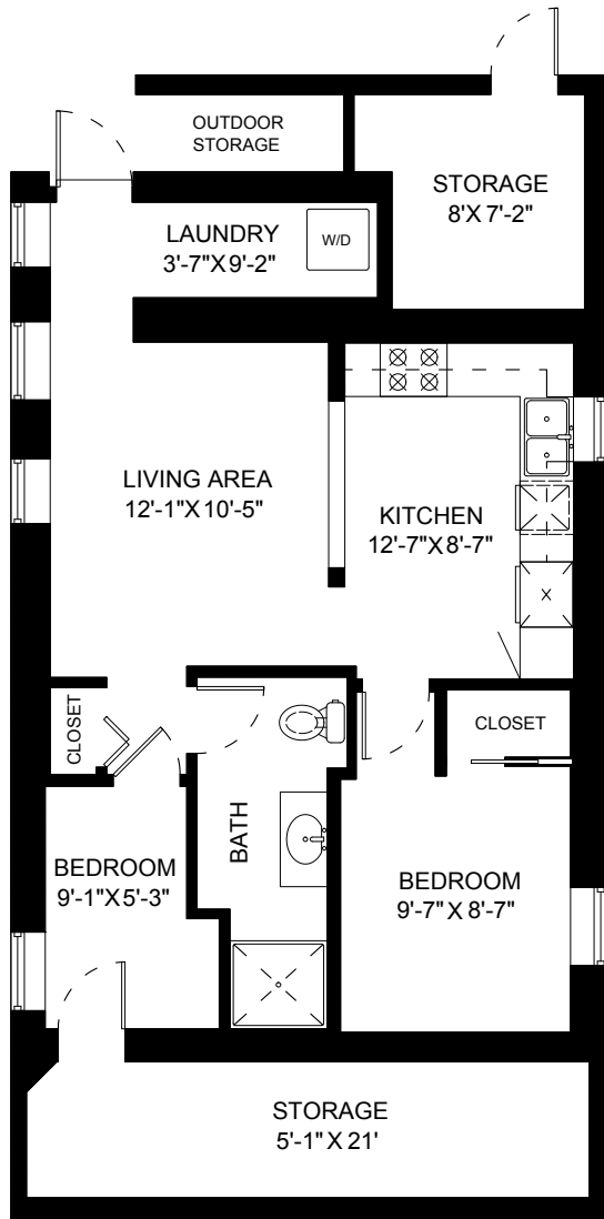
Lower Floor: 831 Sq.Ft. Ceiling Height: 6'-6"
