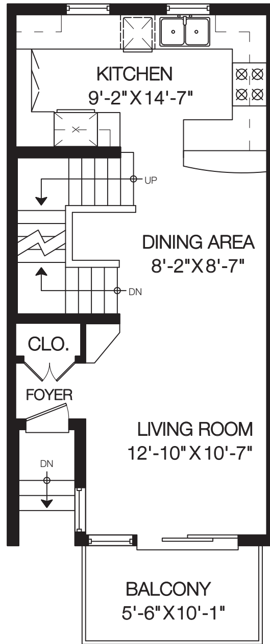
Main Floor: 464 Sq.Ft. Ceiling Height: 9' / Max: 22'-5"
