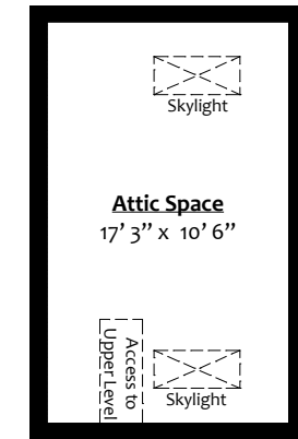
ATTIC (Max CH= 6' 2") Floor Area: 219 Sq. Ft.
