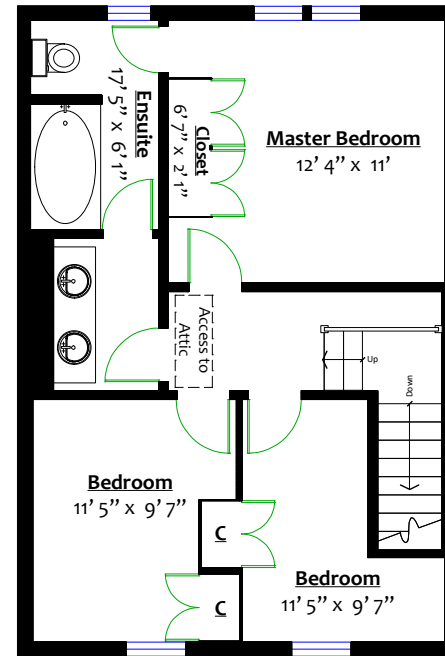
UPPER LEVEL Floor Area: 631 Sq. Ft.
