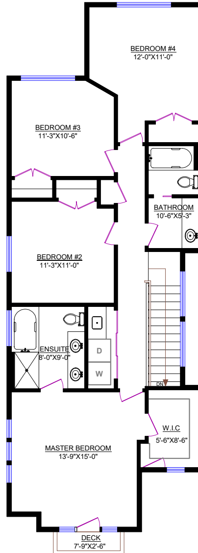
UPPER FLOOR
