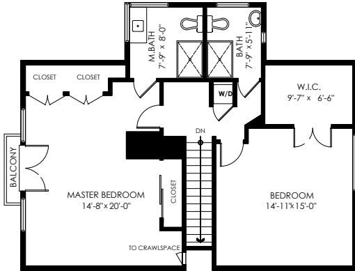
Upper Floor Plan Floor Area: 929 sq.ft. Ceiling Height: 7'-9"
