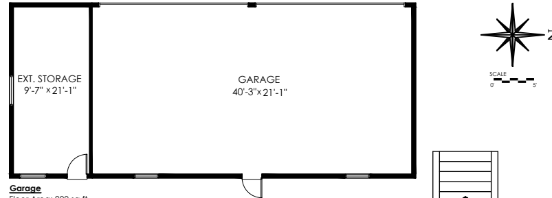
Garage Floor Area: 900 sq.ft. Ext. Storage: 230 sq.ft. Ceiling Height: 8'-6"
