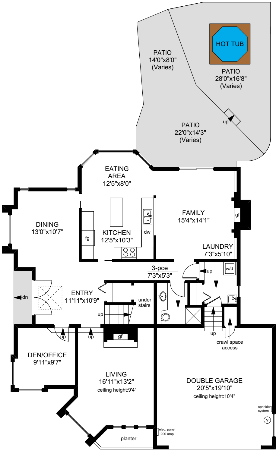
MAIN FLOOR 1415 SQ.FT
