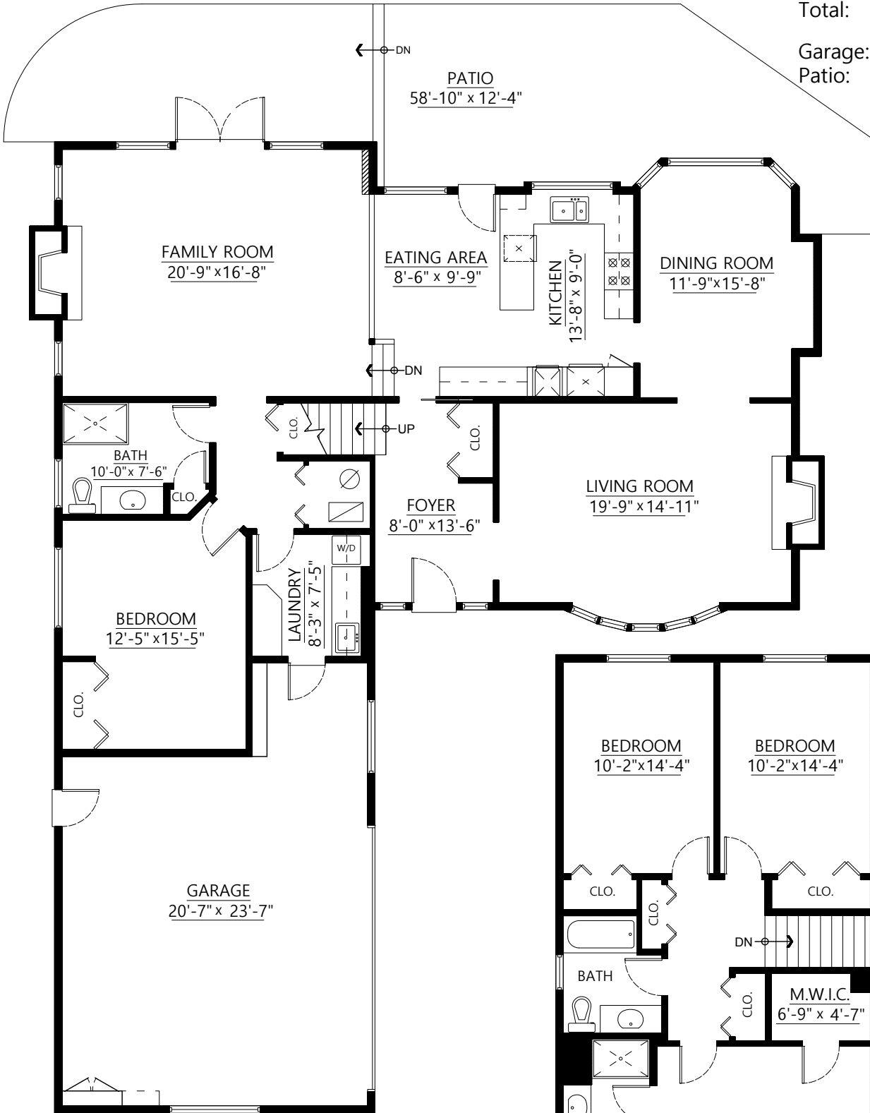
Main Floor Plan Floor Area: 1,700 sq.ft.
