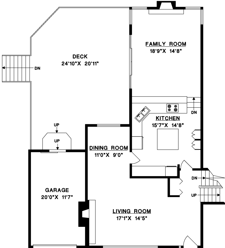
MAIN FLOOR
