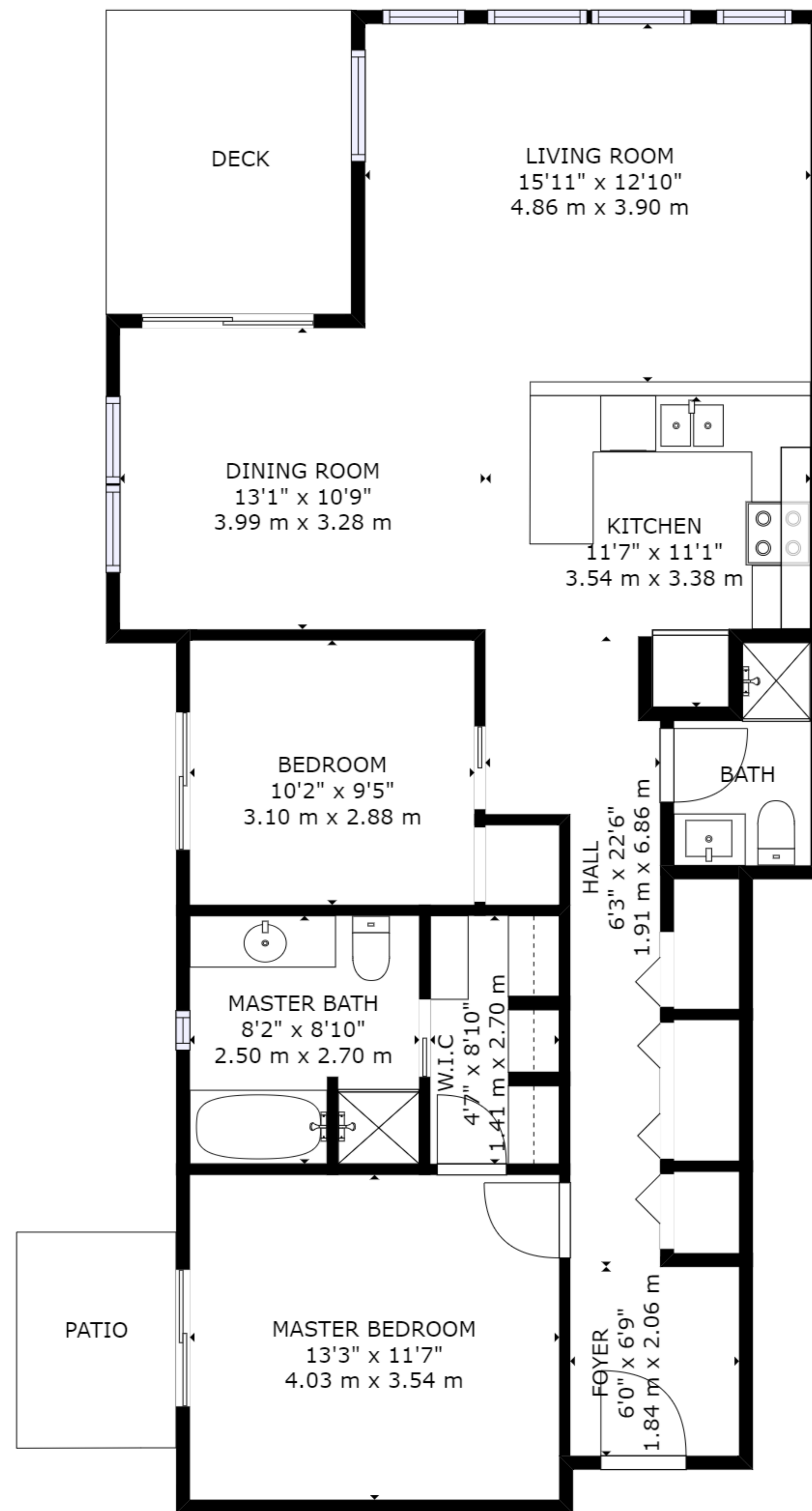
FLOOR 1
