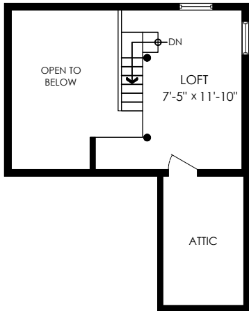
Loft Floor Plan Floor Area: 127 sq.ft. Vaulted Ceiling: 6'-1"
