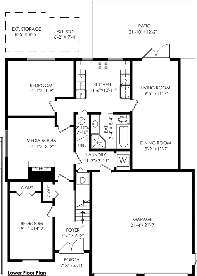
Lower Floor Plan Floor Area: 1232 sq.ft. Ceiling Height: 8'
