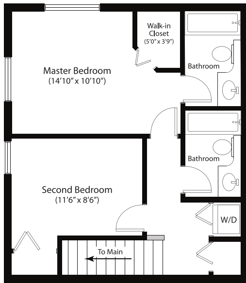
UPPER FLOOR (511 square feet)
