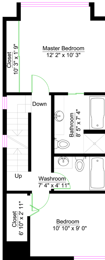
UPPER LEVEL
