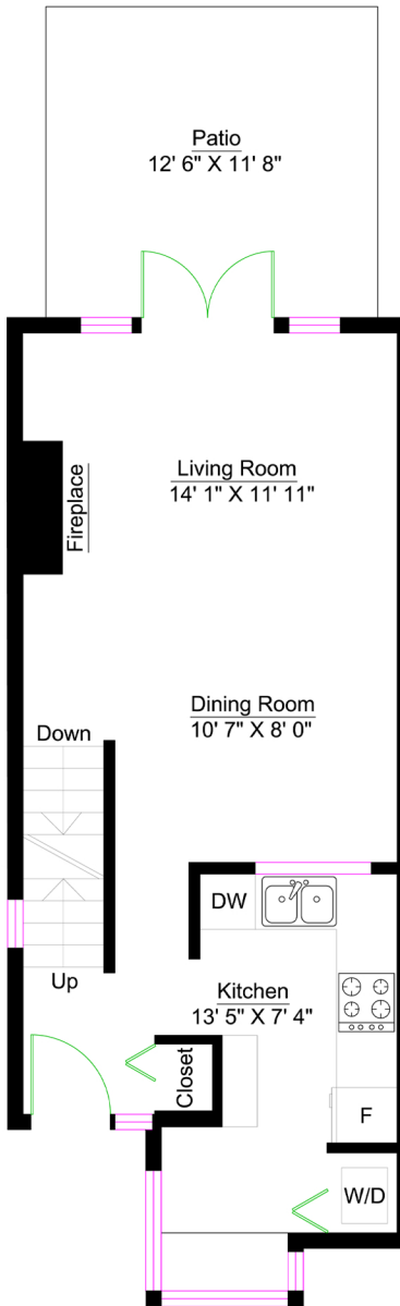
MAIN LEVEL
