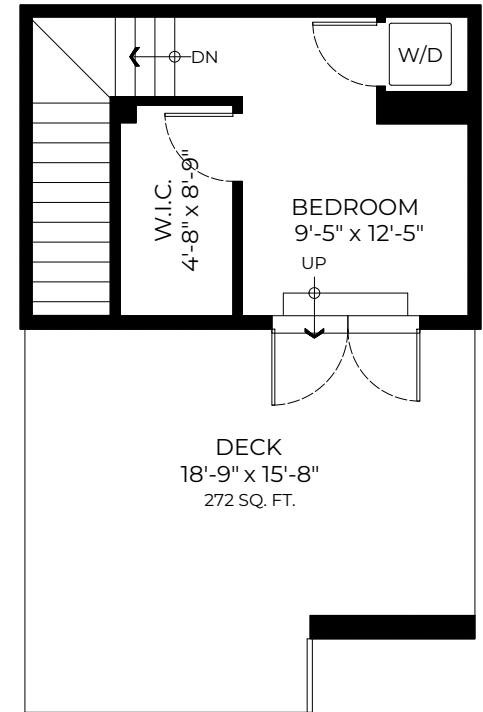
TOP FLOOR PLAN Ceiling Height: 8'-11"
