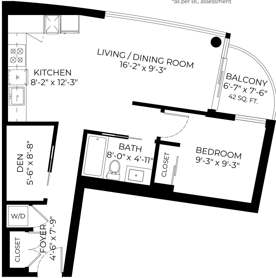
FLOOR PLAN Ceiling Height: 8'-0"
