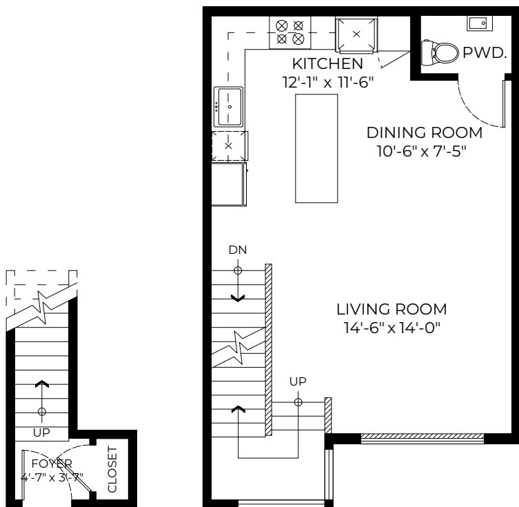
GROUND FLOOR PLAN Ceiling Height: 9'-5"
