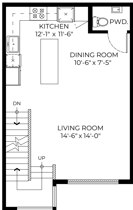
SECOND FLOOR PLAN Ceiling Height: 8'-11"
