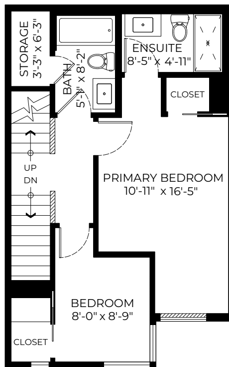
THIRD FLOOR PLAN Ceiling Height: 8'-0"
