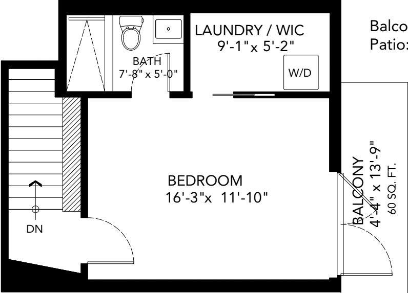
UPPER FLOOR PLAN Ceiling Height: 7'-10"
