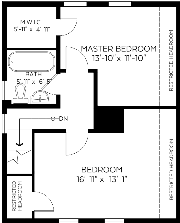
Upper Floor Plan Floor Area: 479 sq.ft.
