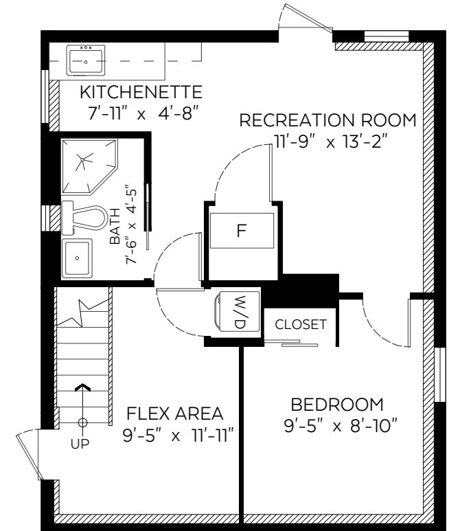
Lower Floor Plan Floor Area: 558 sq.ft.
