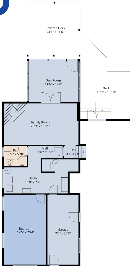
Floor 1
