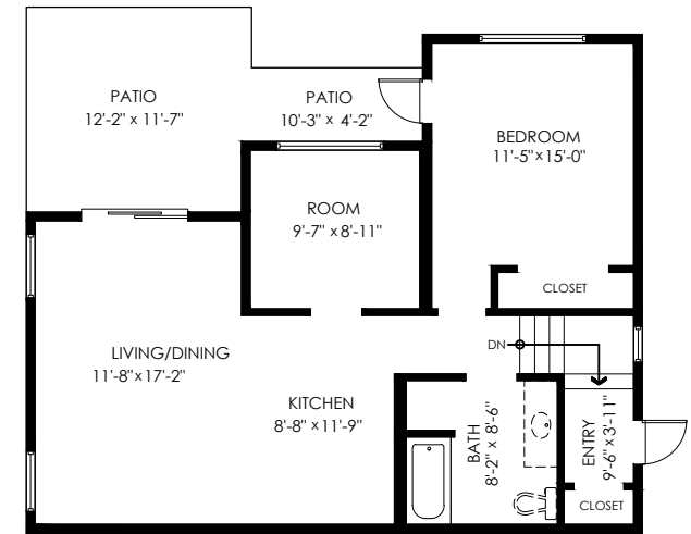
Lower Floor Plan Floor Area: 799 sq.ft. Ceiling Height: 9'-1"
