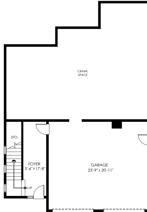
Entry Floor Plan Floor Area: 197 sq.ft.
