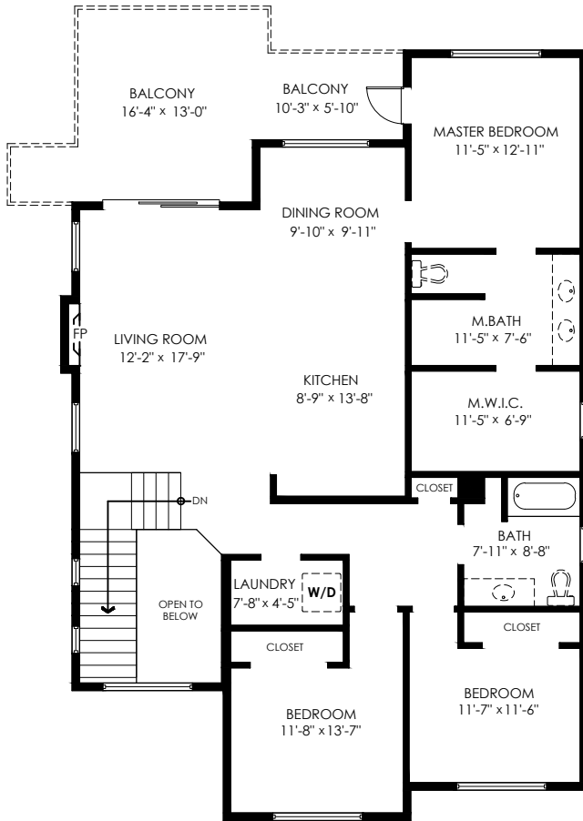
Main Floor Plan Floor Area: 1449 sq.ft. Ceiling Height: 9'-2"
