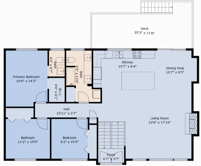
MAIN FLOOR
