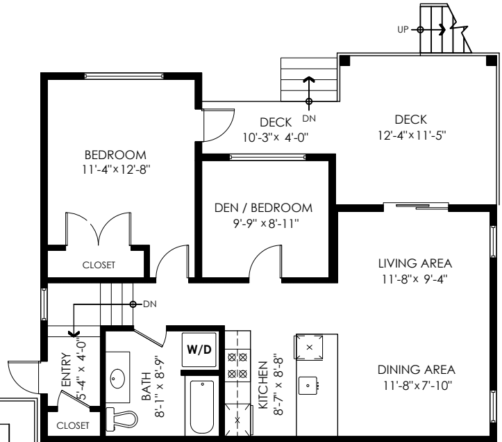
Suite Floor Plan Floor Area: 801 sq.ft. Ceiling Height: 9'
