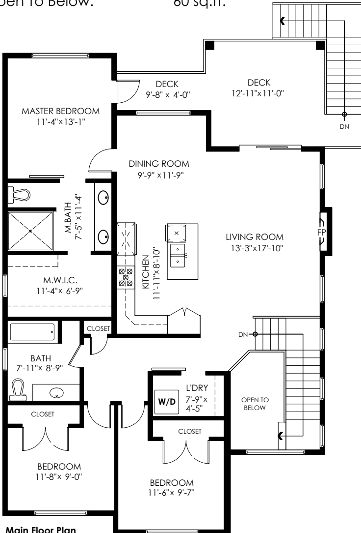
Main Floor Plan Floor Area: 1453 sq.ft. Ceiling Height: 9'-1"
