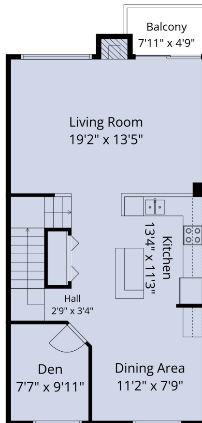
Main Floor
